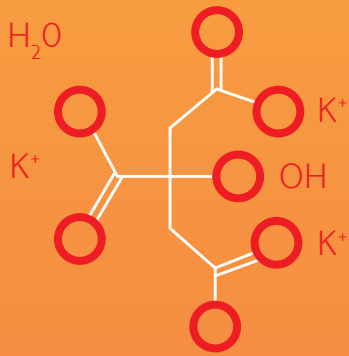
Potassium citrate molecule
